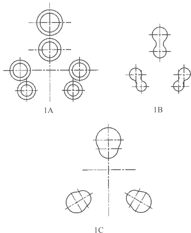
FIG. 1 COMBINED SOCKET-OUTLETS
