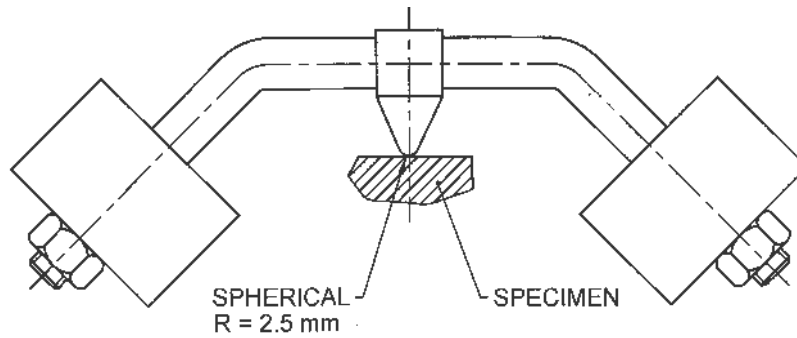
FIG. 38 BALL PRESSURE TEST APPARATUS
